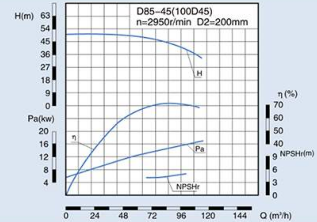
D、DG、DF、DY、MD 85-45(100D45) Performance Data
