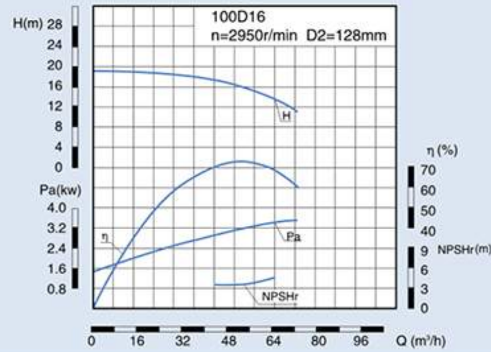
100D、DG、DF、DY、MD16 Performance Data
