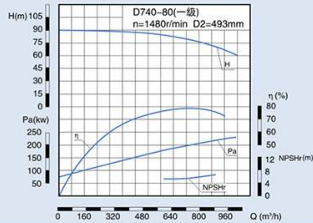
D、DG、DF、DY、MD 740-80 Performance Curve
