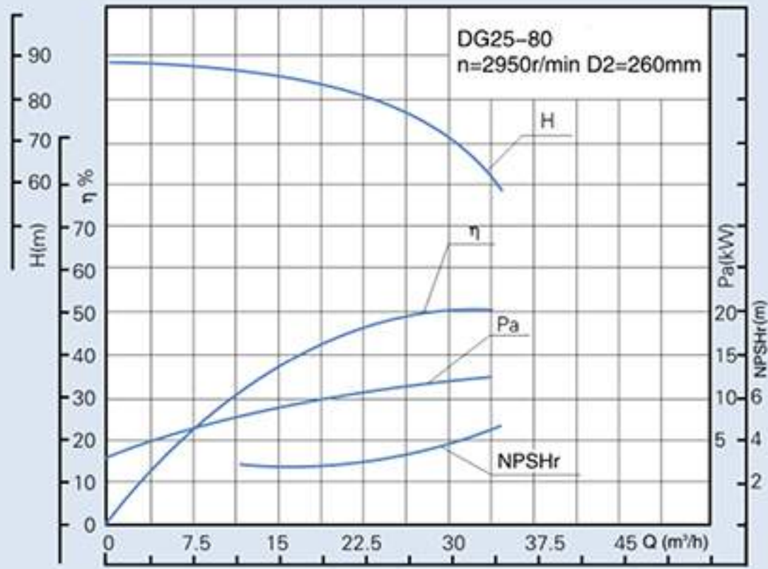
DG25-80 Performance Data
