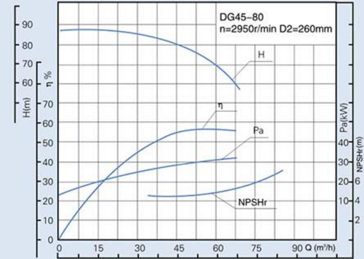
DG45-80 Performance Data
