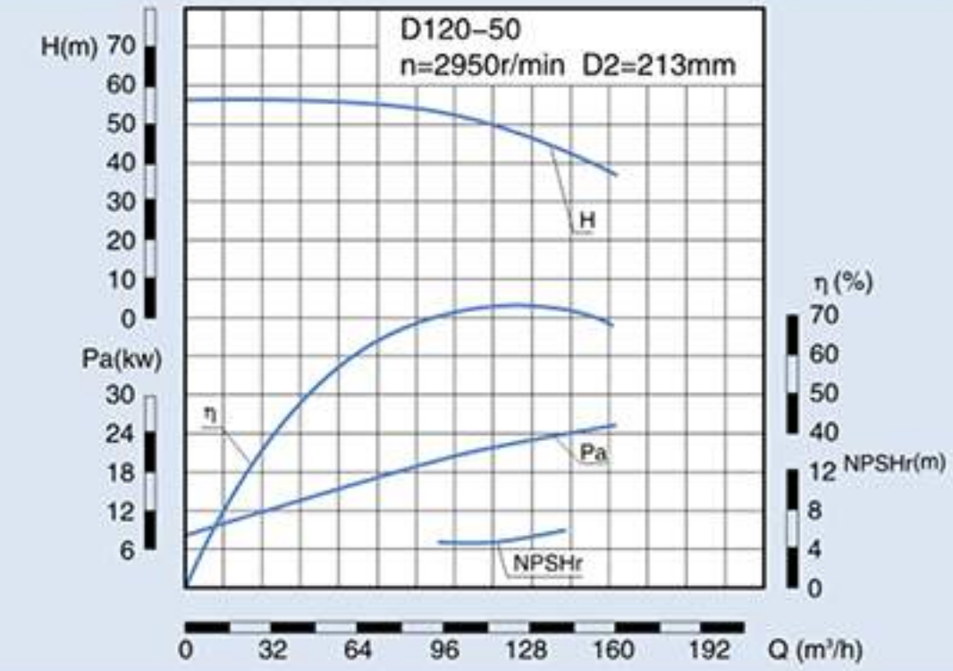
D、DG、DF、DY、MD120-50 Performance Data
