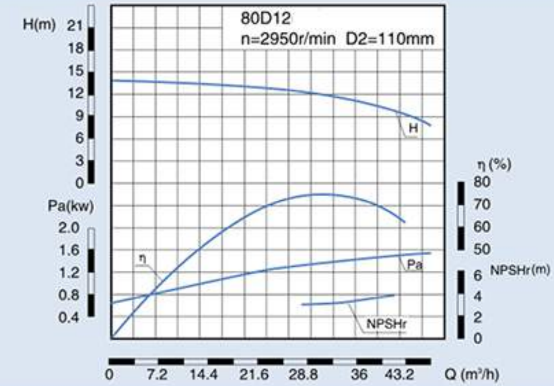
80D、DG、DF、DY、MD12 Performance Data
