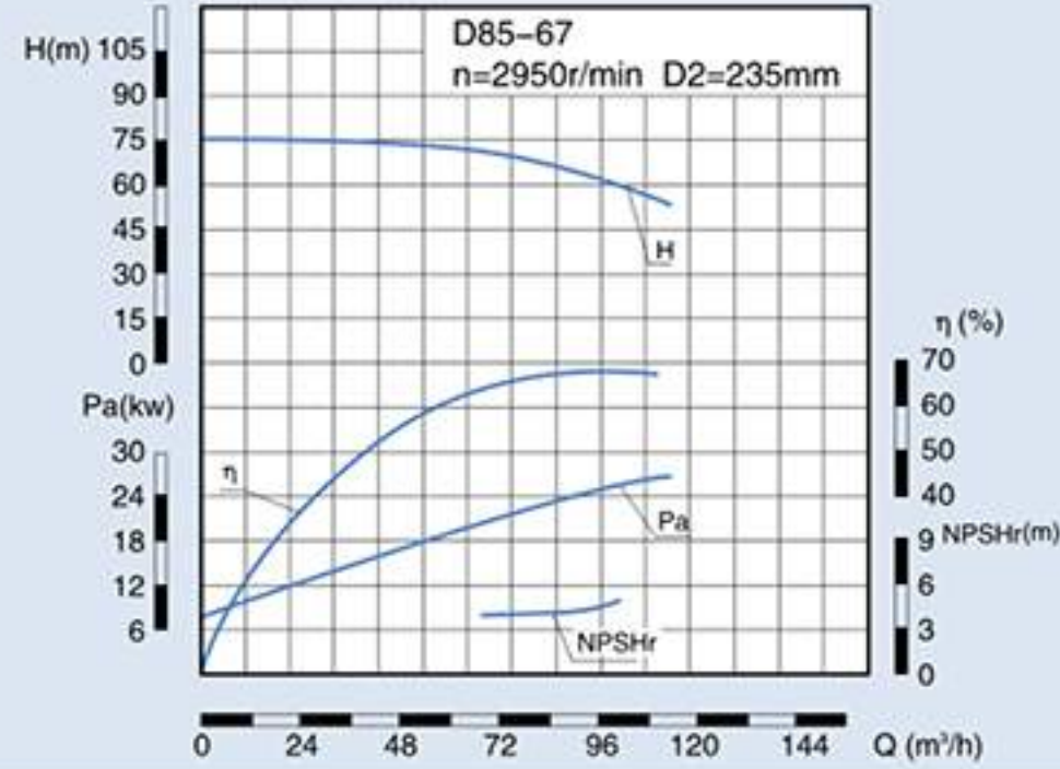
D、DG、DF、DY、MD85-67 Performance Data
