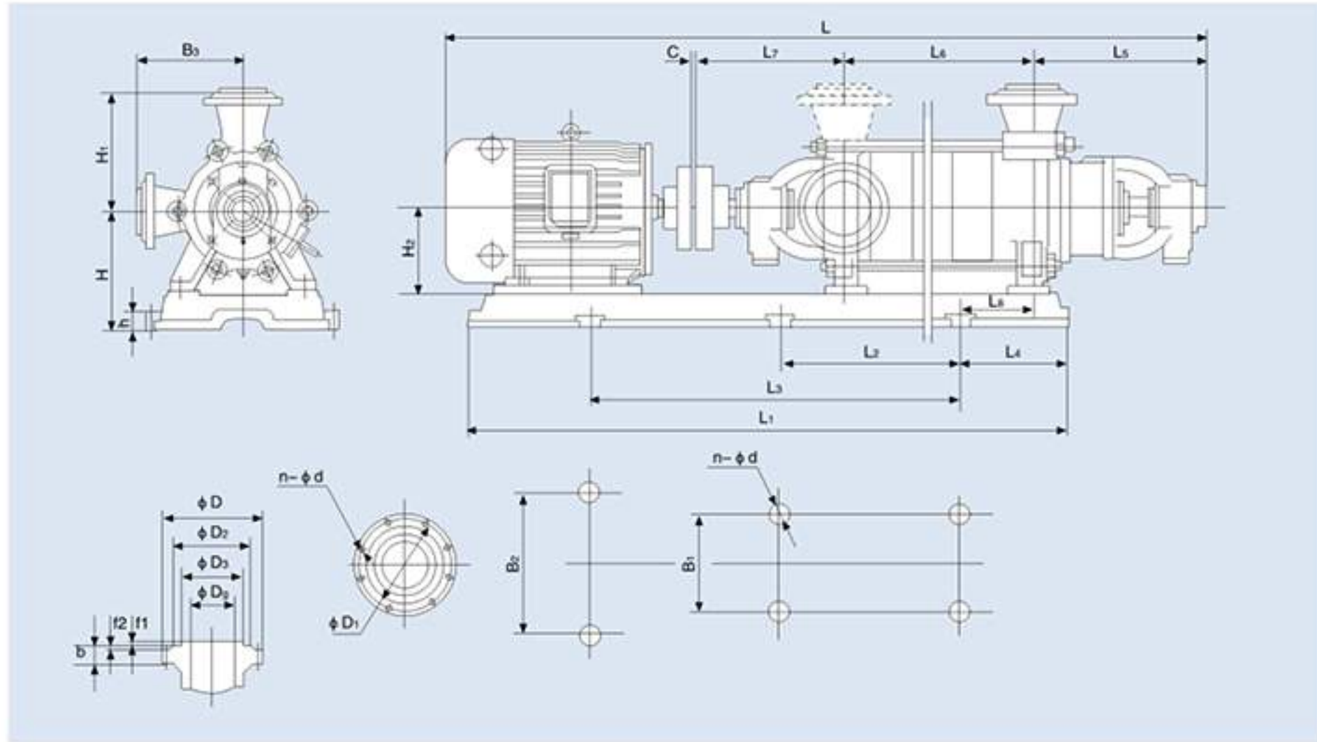
D、DG、DF、DY、MD (With Pump Base)
