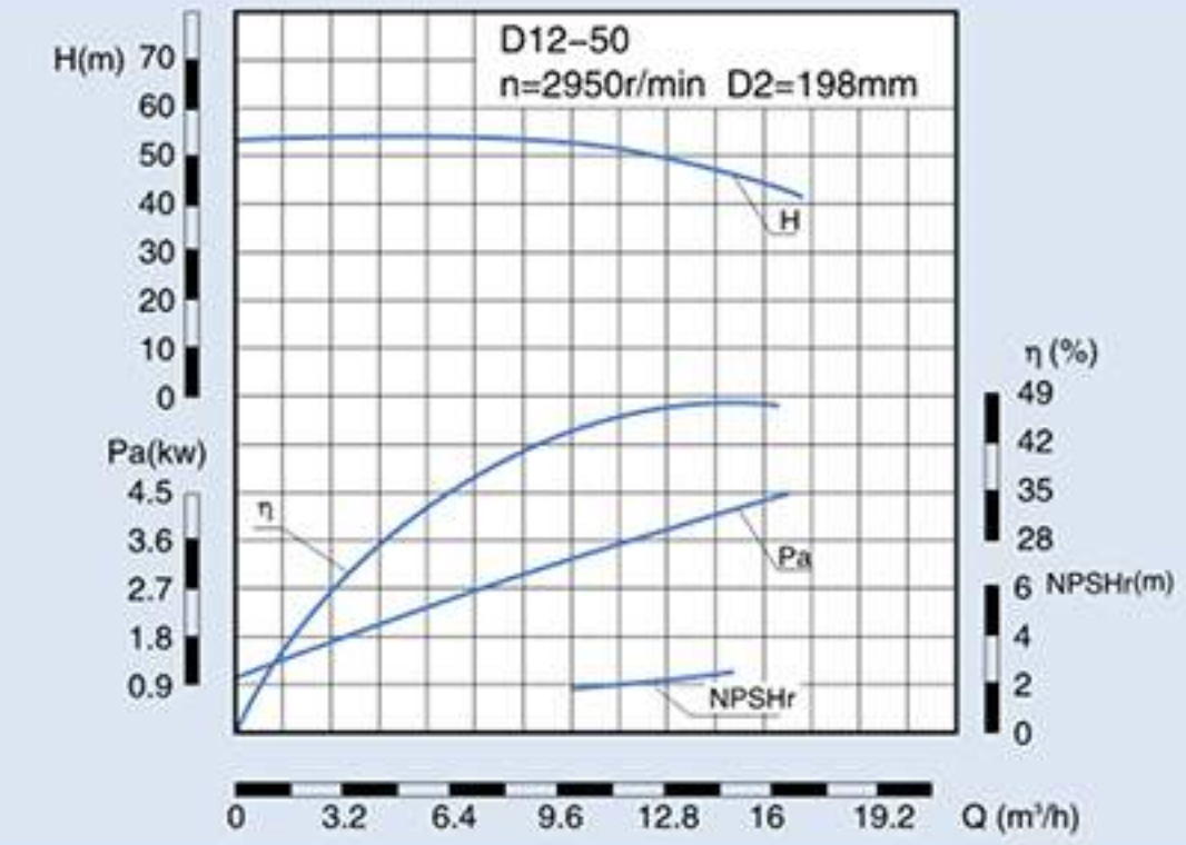
D、DG、DF、DY、MD12-50 Performance Data
