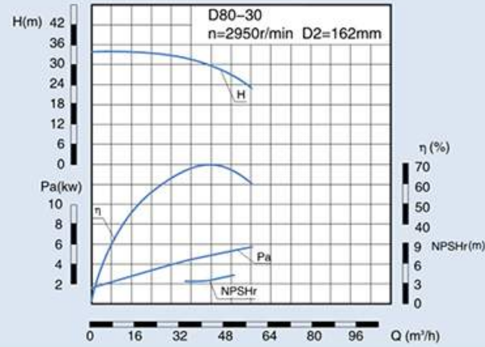
D、DG、DF、DY、MD80-30 Performance Data
