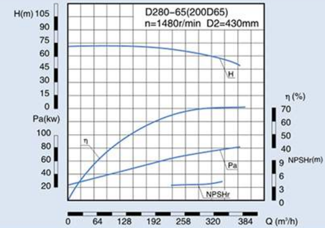
D、DG、DF、DY、MD280-65(200D65) Performance Data
