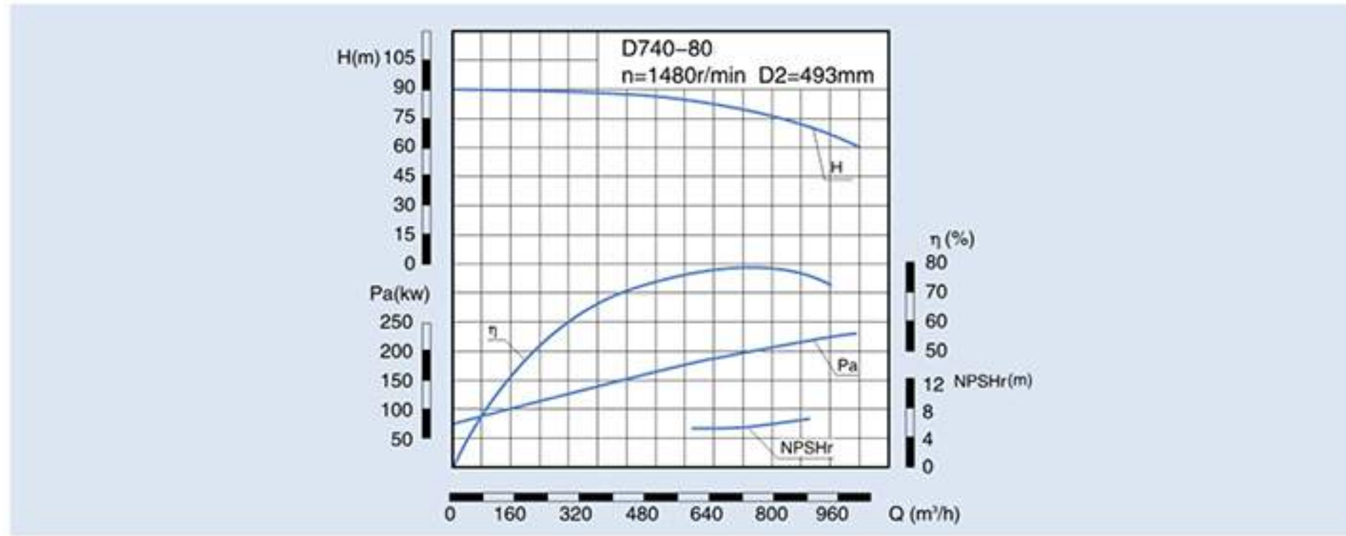
D、DG、DF、DY、MD 740-80 Performance Curve
