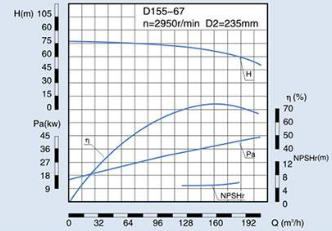
D、DG、DF、DY、MD155-67 Performance Data
