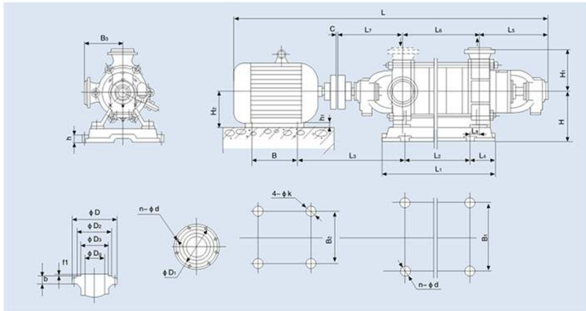
D、DG、DF、DY、MD (With Pump Base)
