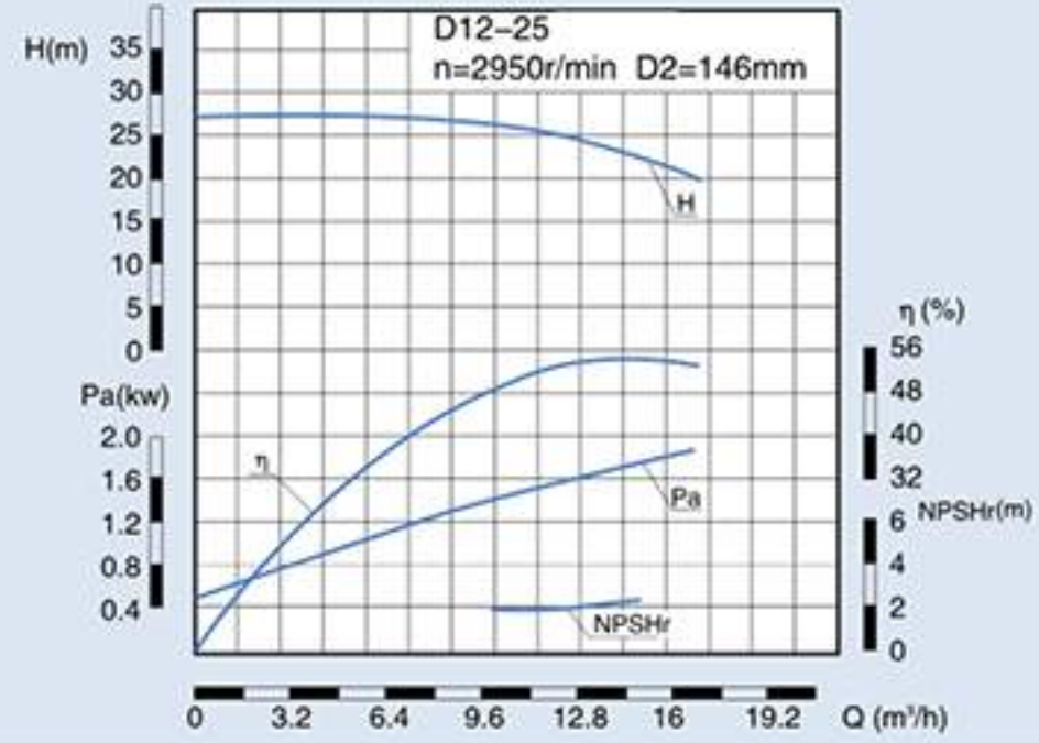
D、DG、DF、DY、MD12-25 Performance Data
