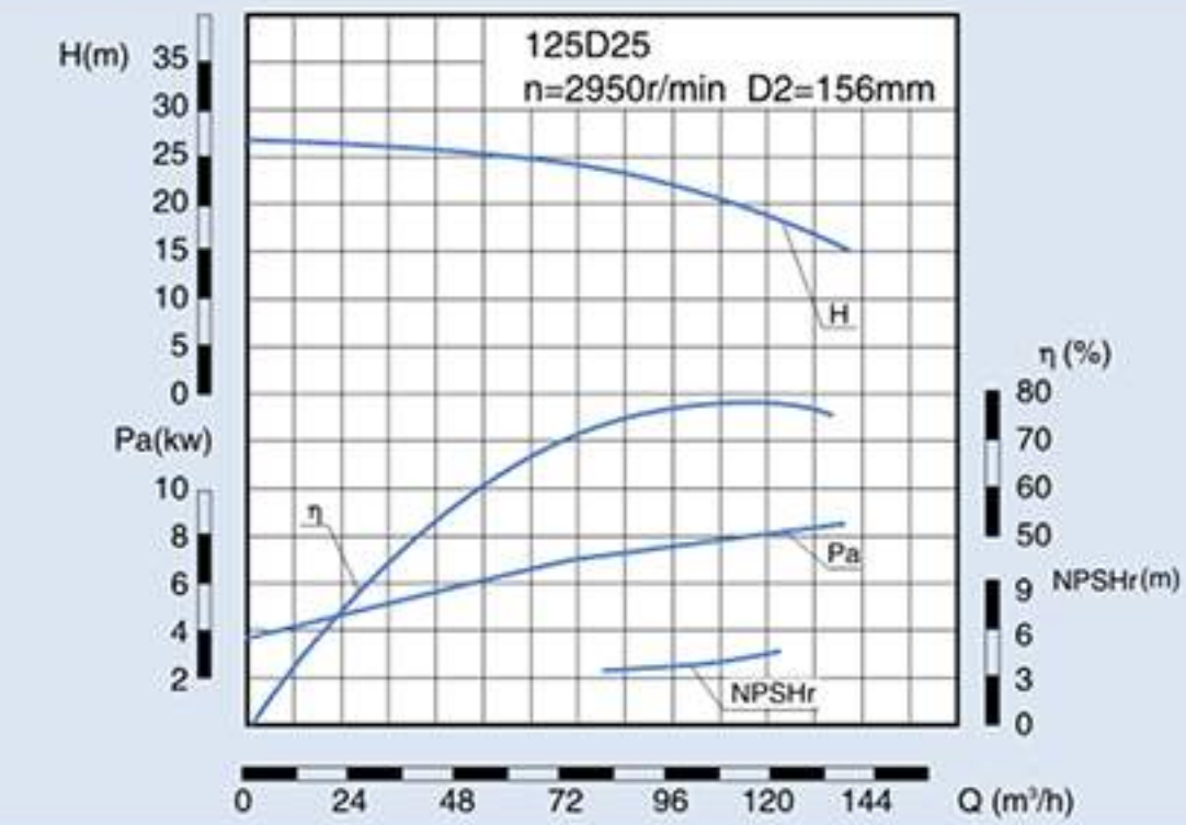
125D、DG、DF、DY、MD25 Performance Data
