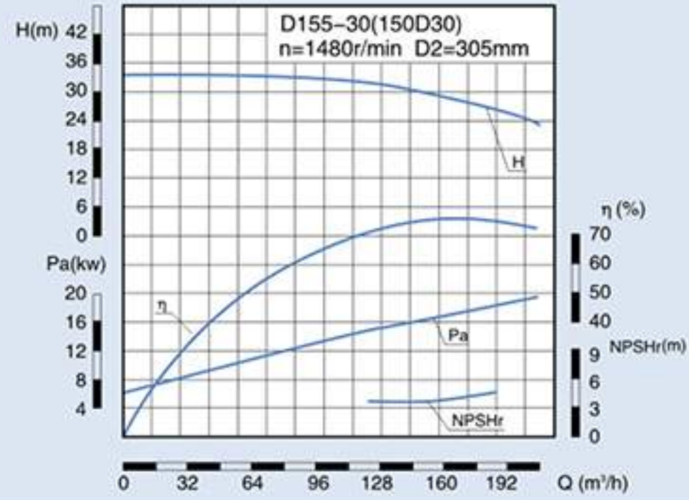
D、DG、DF、DY、MD 155-30(150D30) Performance Data
